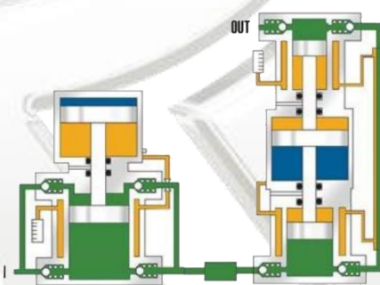
Model AGD-4 feeding into/Model AGT
